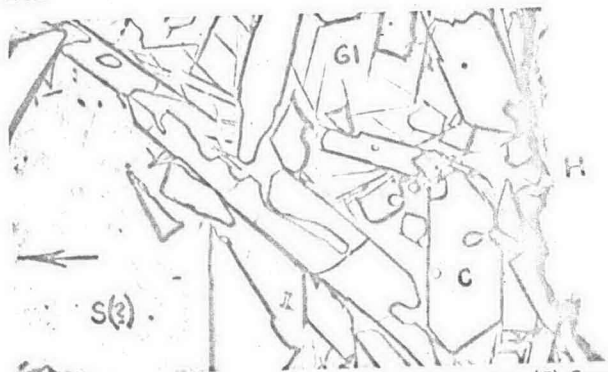
Fig. 2. Effect of temperature gradient across sample. (C) Corundum, (S) sillimanite (?), (G) glass, and (H) higher-temperature side near the heater. Arrow indicates direction to center of cell. (As polished, bright field, \times 390 .)
